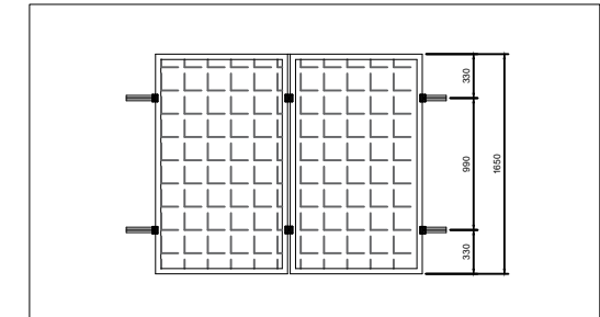
Portrait Panel Orientation 60 Cell
