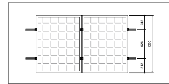
Portrait Panel Orientation 170 W
