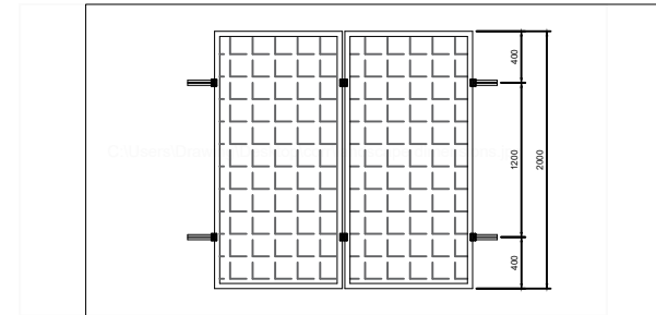
Portrait Panel Orientation 72 Cell
